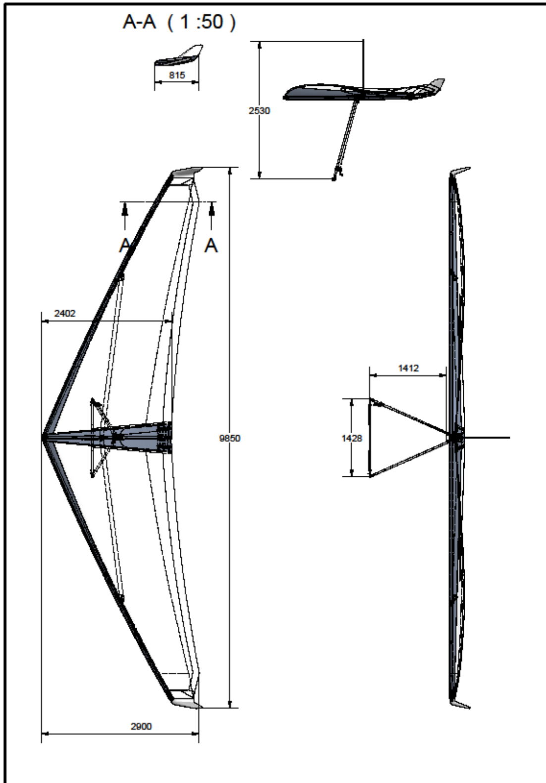
Figure 3-1: BioniX in 3 Perspectives
